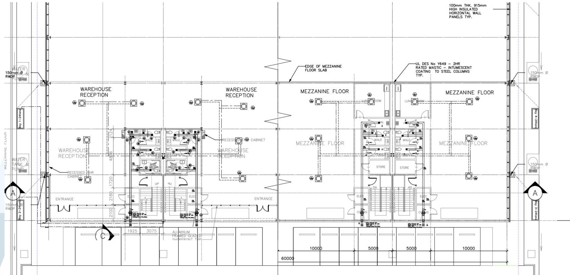
1 GROUND FLOOR VAC LAYOUT SCALE: 1:100
